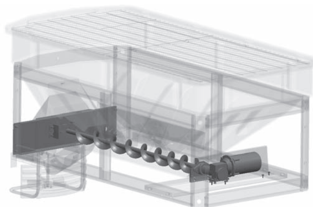
Auger Drive Assembly
